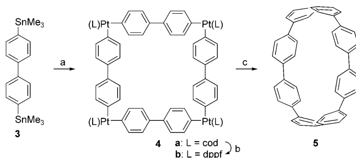
Scheme 2. Synthesis of 5 . Reaction conditions and reagents: a) [PtCl 2 (cod)] (1 equiv), THF, reflux, 35 h, 57%. b) dppf (4.0 equiv), CH 2 Cl 2 , RT, 20 h, 91%. c) Br 2 (7 equiv), toluene, 95°C, 17 h, 49%.
